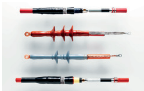
LV and MV power cable accessories of different technologies, as e.g. heat-shrinkable, cold-shrinkable, pre-molded, resin and tape based solutions
