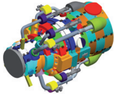
Insulation pillows for 70MW gas turbines
