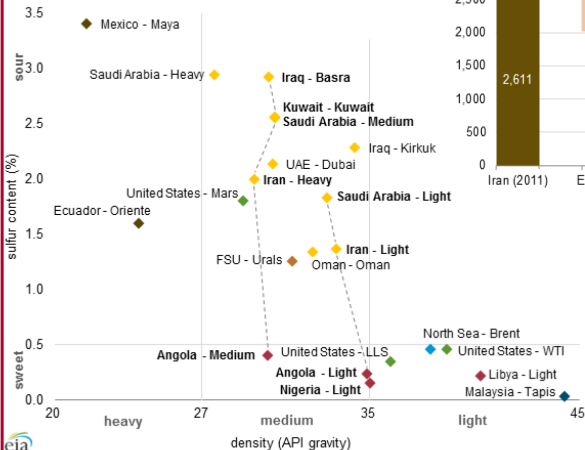
Density and sulfur content of selected crude oils
