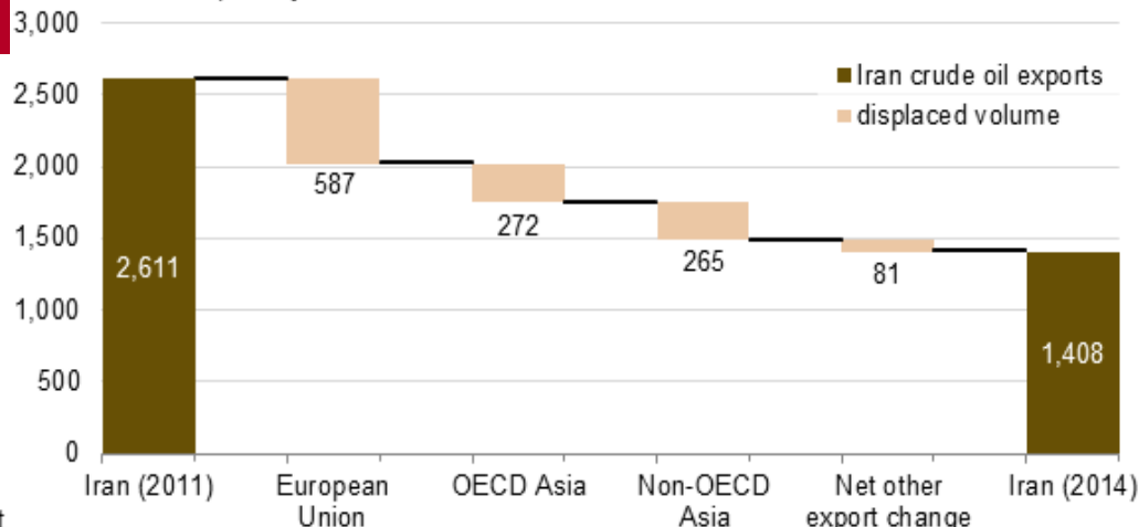
Iran crude oil exports by destination (2011-14) thousand barrels per day
